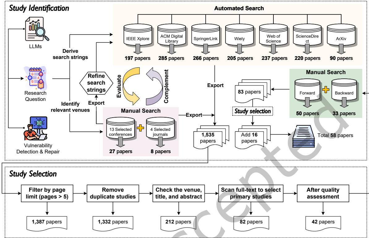
Fig. 2. Study Identification and Selection Process
